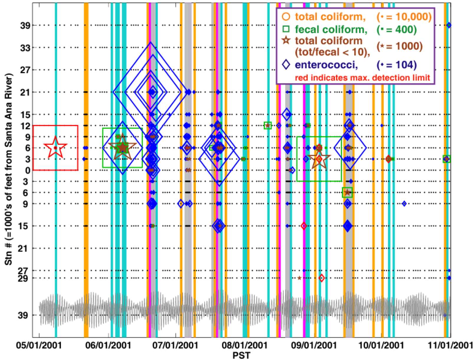
Figure 2. The vertical bars indicate days on which bacterial events occurred, blue = type 1, magenta = type 2, gray = types 1 and 2, gold = type 3. Sea level measured at Los Angeles is shown at the bottom of the figure. A black dot is plotted at each time and location a sample was taken. Colored symbols are plotted at the time and location of samples exceeding AB411 single sample standards. The size of the symbol is proportional to the ratio of the measured bacterial concentration to the AB411 criteria. The symbol size for a sample equal to the AB411 criteria is shown to the right of the indicator species in the legend.
